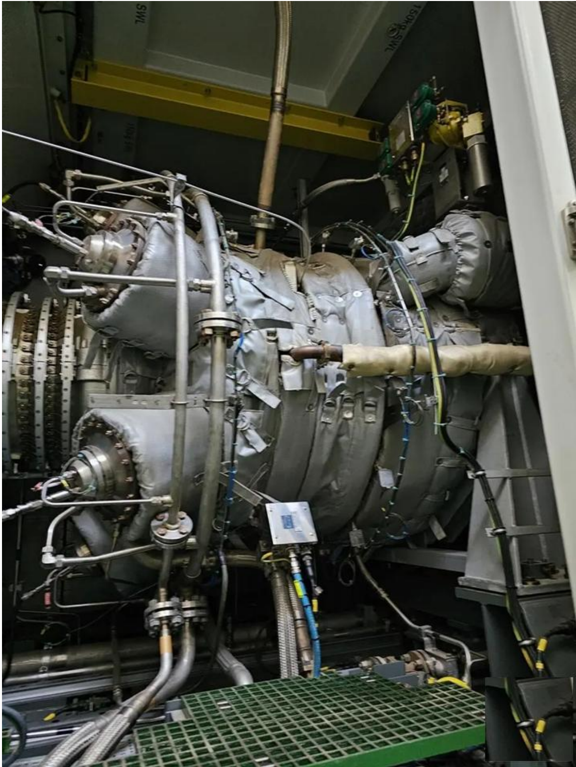
2 units of Siemens SGT-400 DLE — 14.4 MW,60HZ Twin-Shaft Gas-Turbine Package (2019 • very low working hours).
